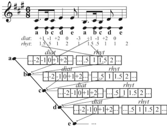
Figure 4. Progressive construction of pattern abcde and of its two occurrences, by storing the intervals in hash tables associated with each successive state of the pattern.
